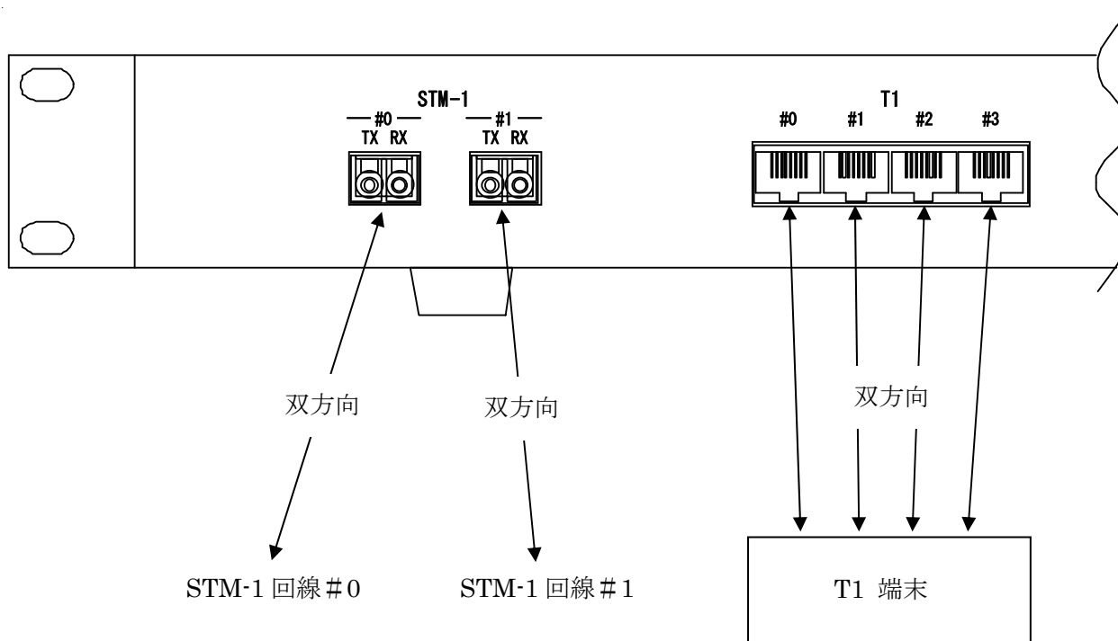
STM1-T1×4 Convertor
